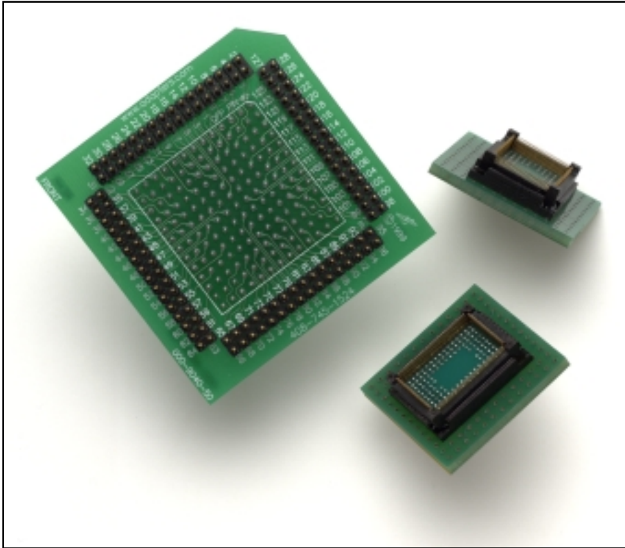
The Delta-Clip, High density Clip-on adapters
